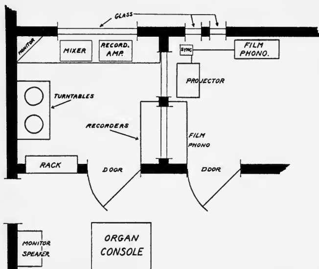
FIG. 3. Layout of recording and projection rooms.
